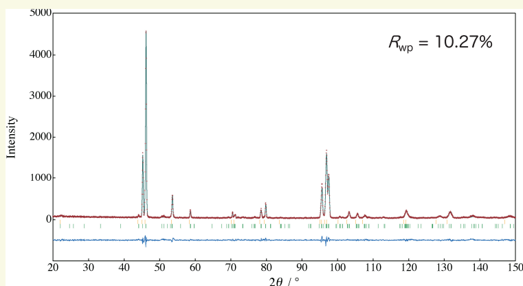
図1 \text{Li}(\text{Li},\text{Mn})_{1-x}\text{Co}_x\text{O}_2 系( x = 0.1 )のRietveld解析結果
